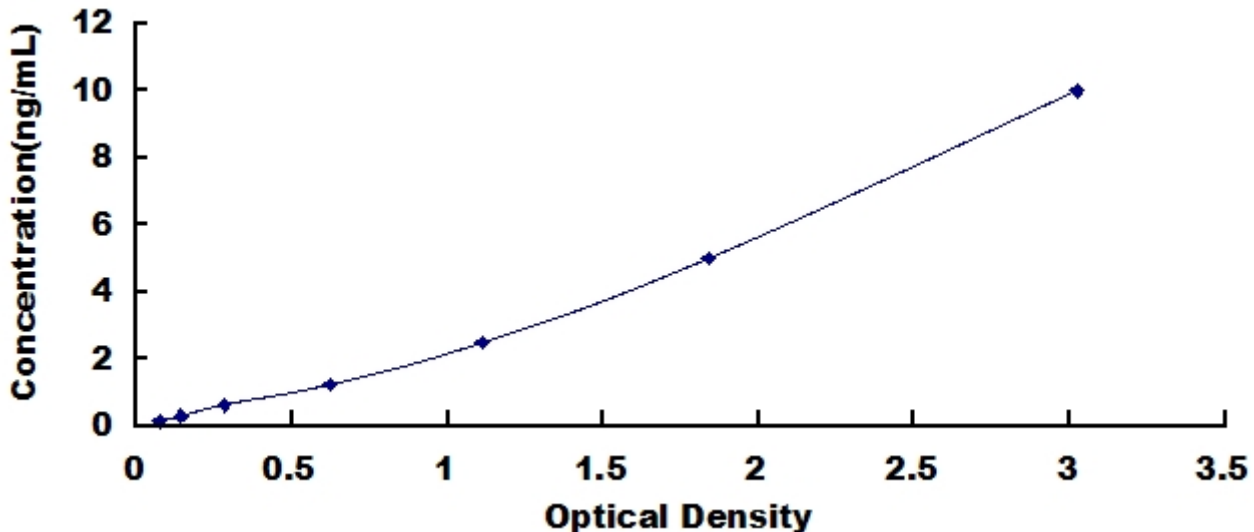
Typical Standard Curve for Thromboxane Receptor, Human ELISA.
