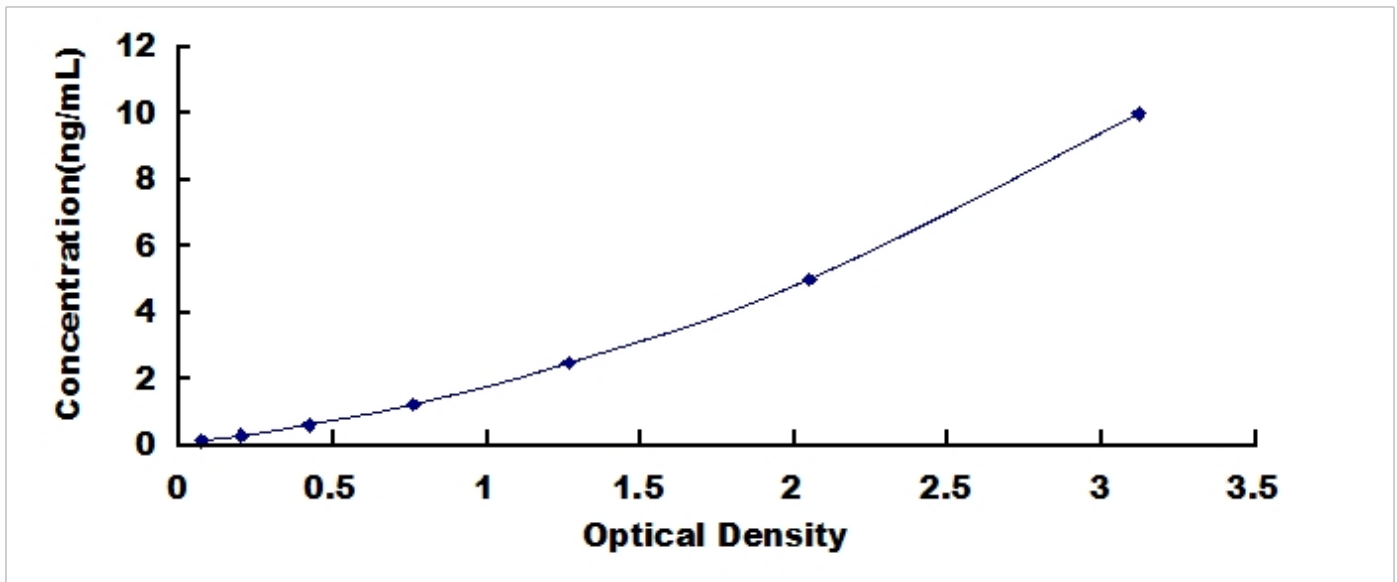
Typical Standard Curve for TOP2b, Human ELISA.
