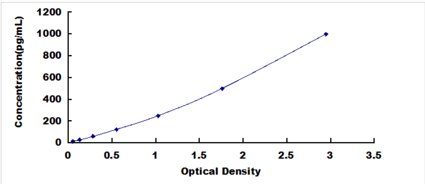
Typical Standard Curve for TGFb2, Caprine ELISA.
