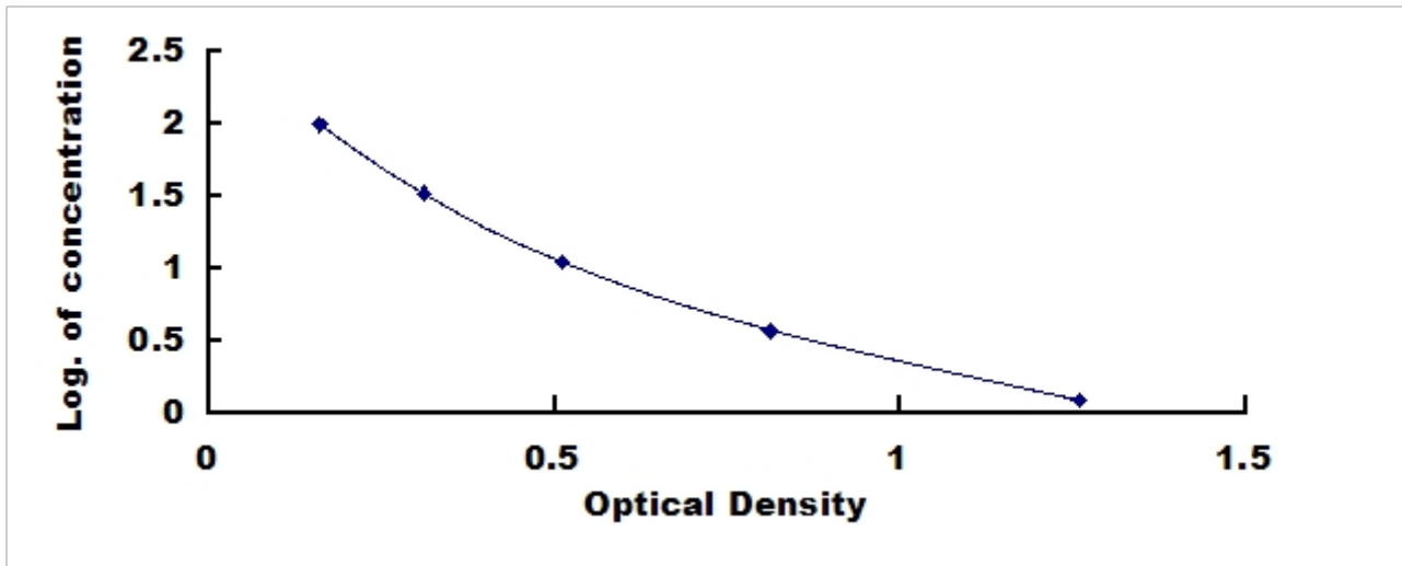
Typical Standard Curve for Tryptophan ELISA.
