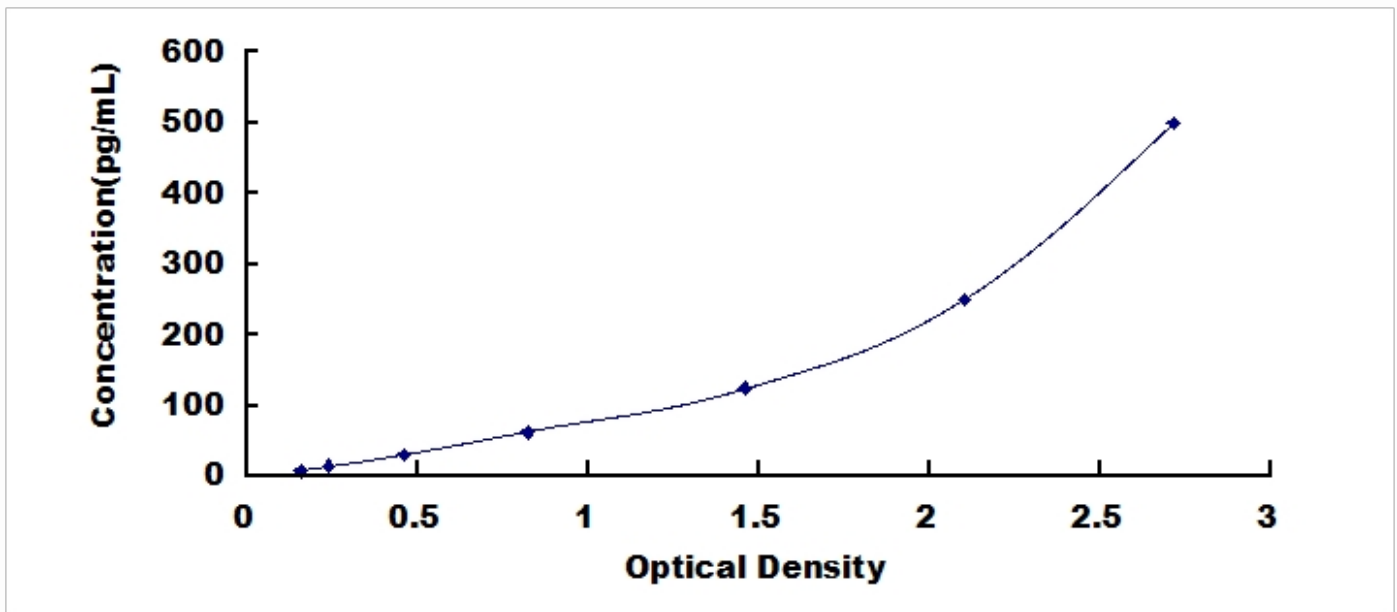
Typical Standard Curve for TNFa, Cavia ELISA.
