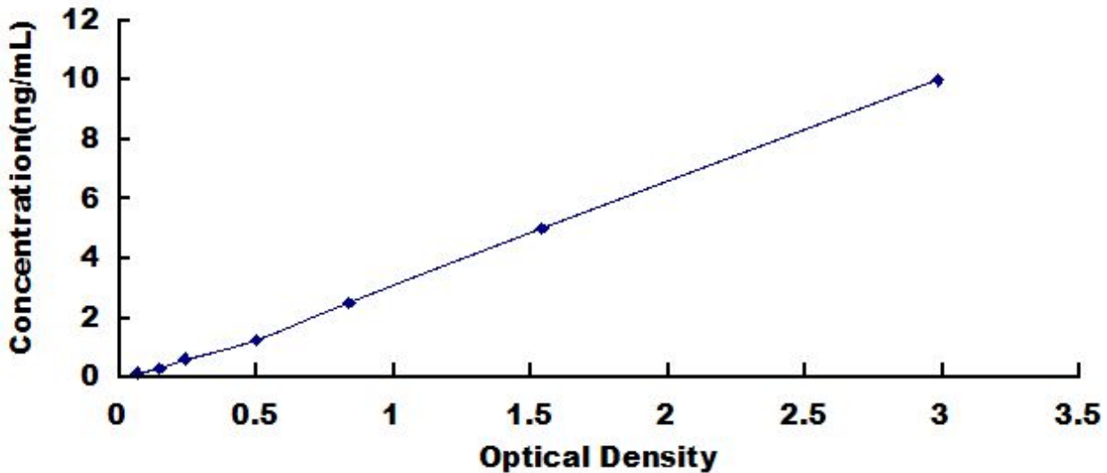
Typical Standard Curve for TRAIL, Canine ELISA.
