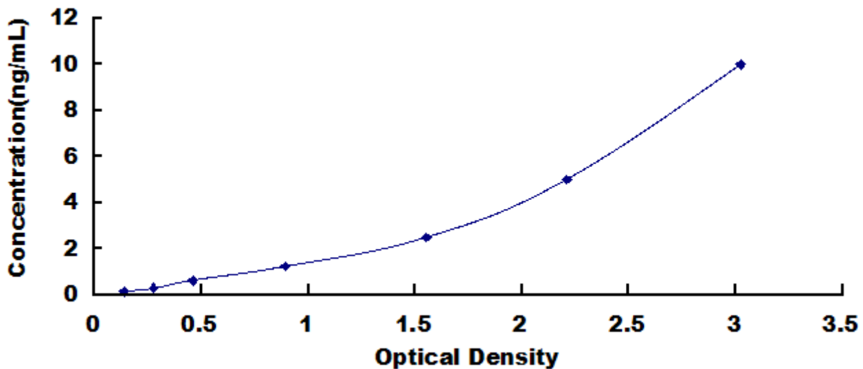
Typical Standard Curve for TWSG1, Human ELISA.
