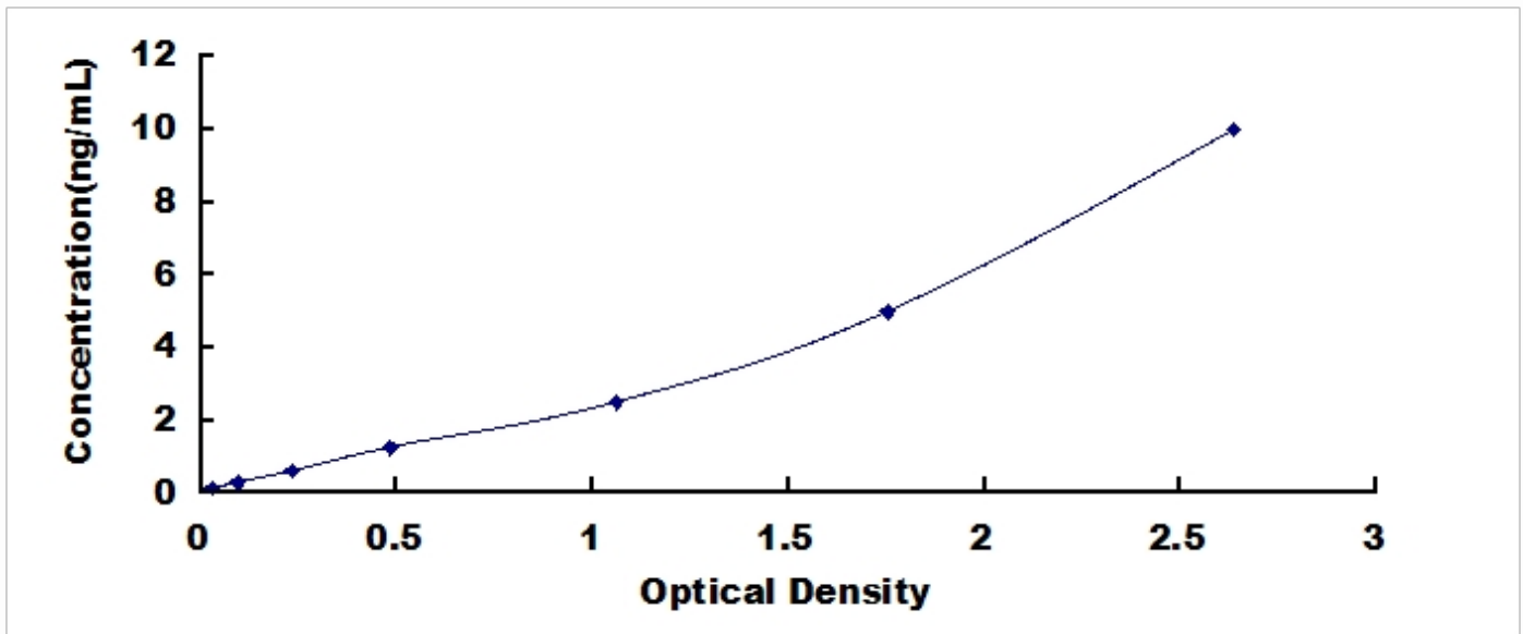
Typical Standard Curve for Tyrosine Hydroxylase, Rat ELISA.
