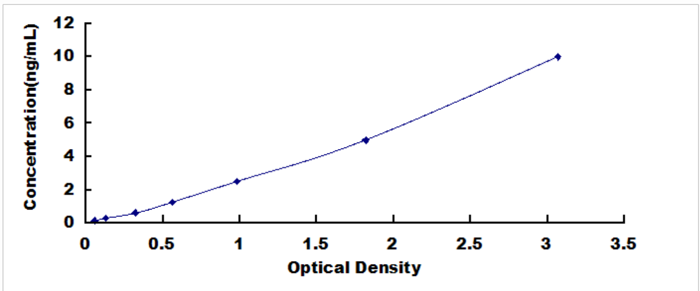
Typical Standard Curve for VRK1, Human ELISA.
