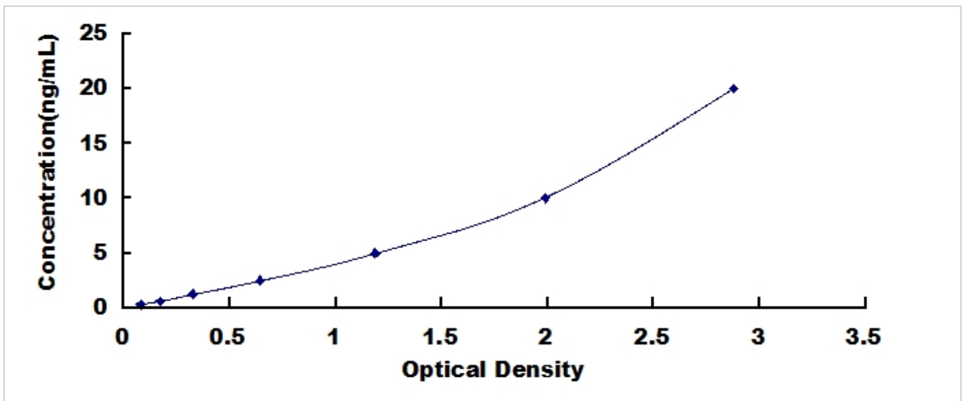
Typical Standard Curve for VNN3, Mouse ELISA.
