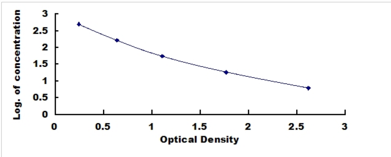
Typical Standard Curve for VIP, Rat ELISA.
