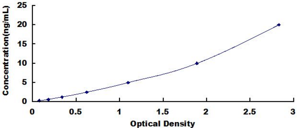
Typical Standard Curve for Vasorin, Mouse ELISA.
