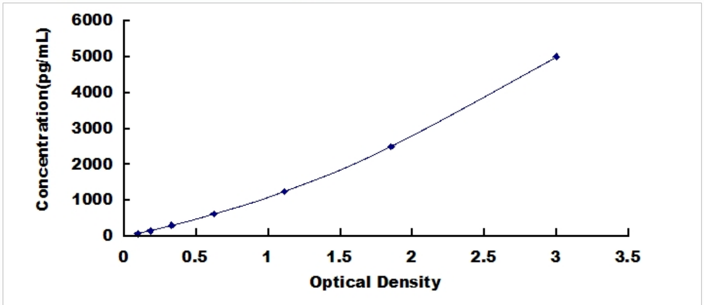
Typical Standard Curve for VGLL1, Human ELISA.
