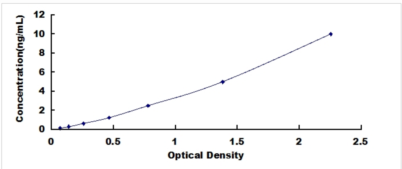
Typical Standard Curve for WNT3, Rat ELISA.
