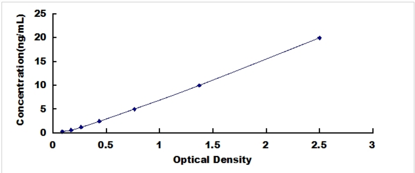
Typical Standard Curve for WFS1, Rat ELISA.
