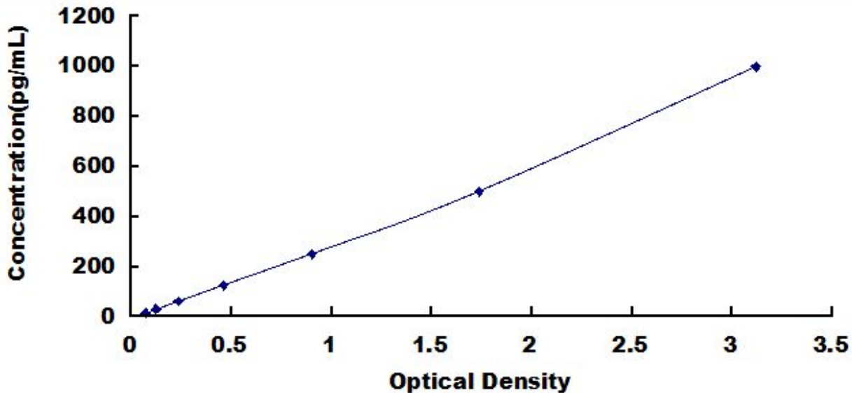
Typical Standard Curve for cTnI, Human ELISA.
