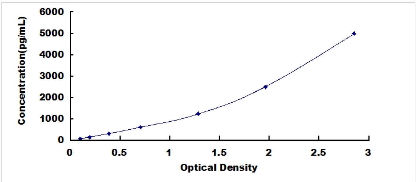
Typical Standard Curve for HSPD1, Human ELISA.
