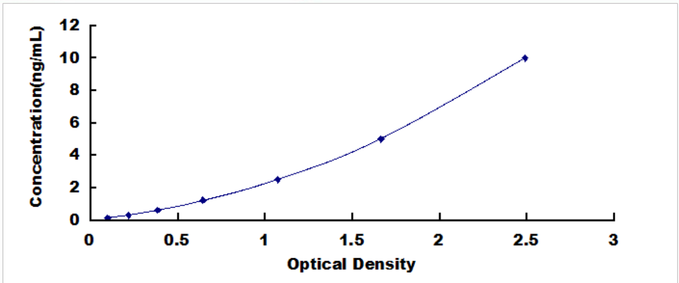
Typical Standard Curve for Hepcidin, Mouse ELISA.
