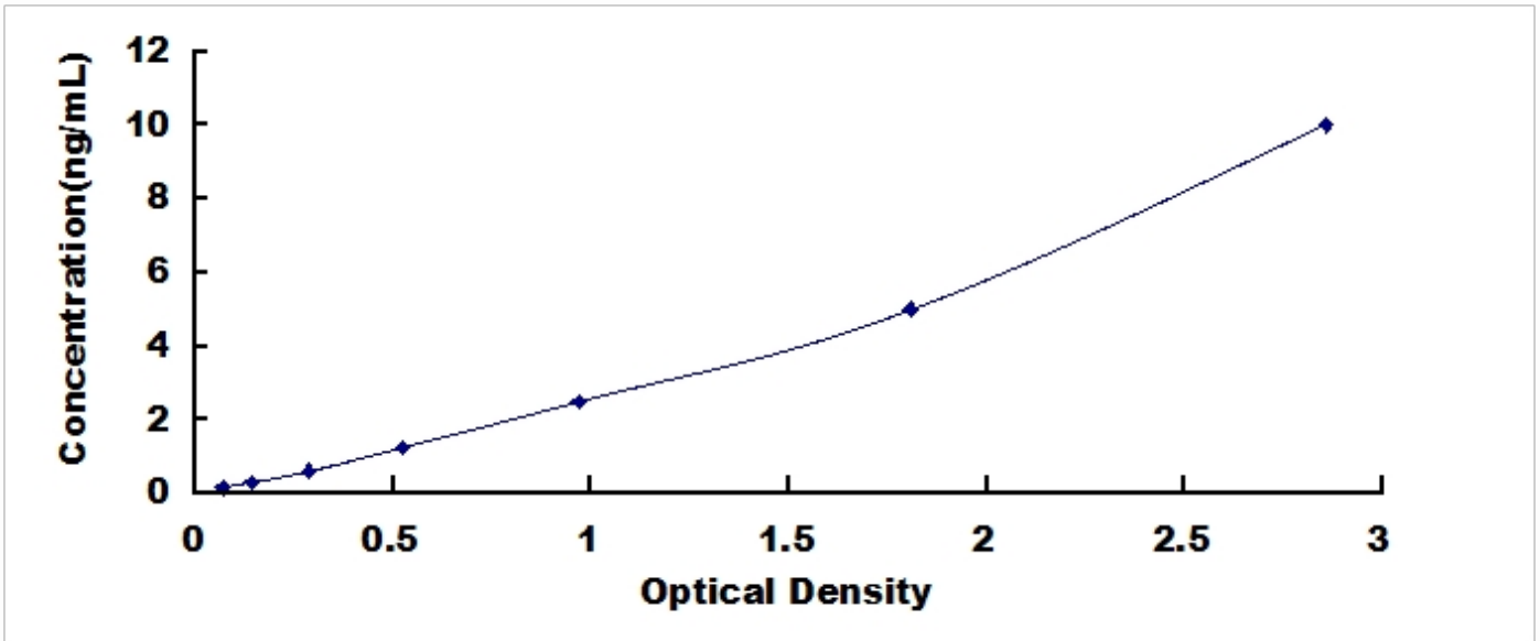
Typical Standard Curve for IgG, Bovine ELISA.
