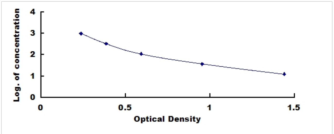
Typical Standard Curve for Malondialdehyde ELISA.
