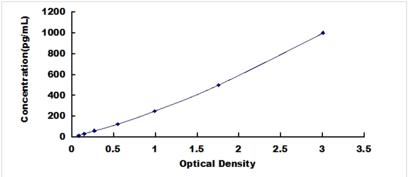
Typical Standard Curve for PER1, Human ELISA.
