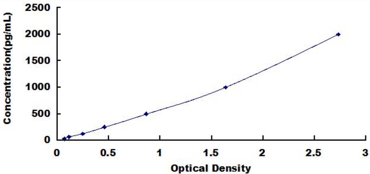
Typical Standard Curve for PRNP, Human ELISA.
