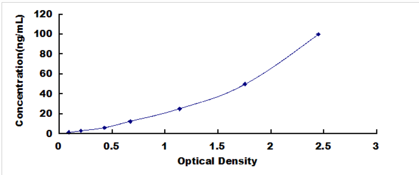
Typical Standard Curve for Prolactin, Porcine ELISA.
