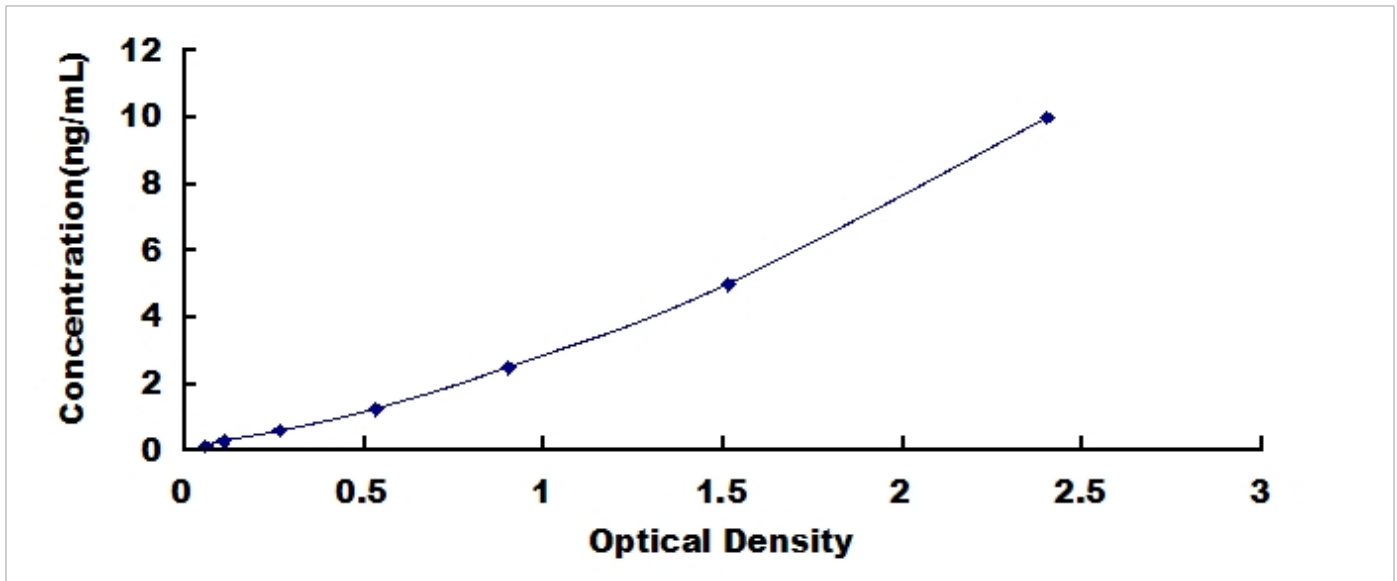
Typical Standard Curve for WNT3A, Human ELISA.
