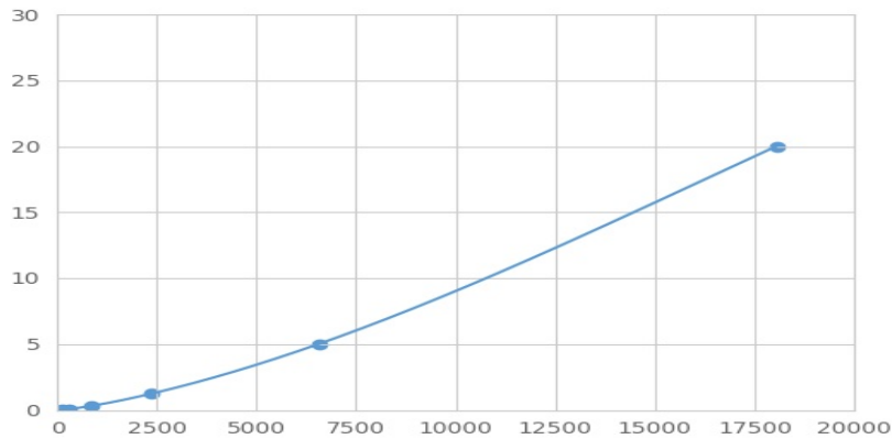
Typical Standard Curve for HSD17b3 Magnetic Luminex Assay.
