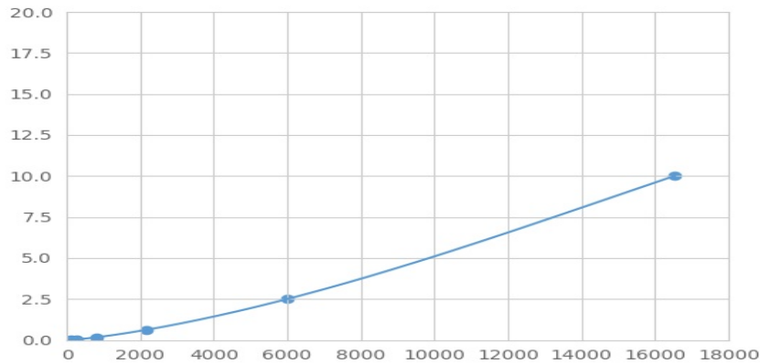
Typical Standard Curve for ADAMTS7 Magnetic Luminex Assay.
