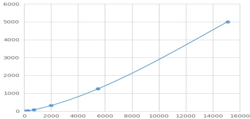
Typical Standard Curve for ABCA7 Magnetic Luminex Assay.
