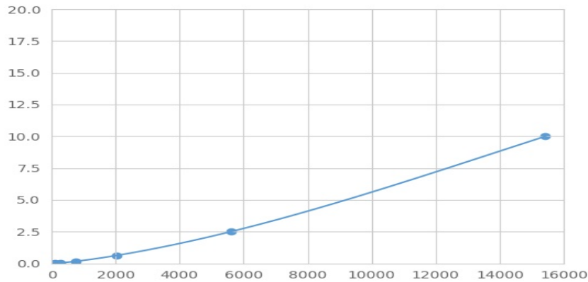
Typical Standard Curve for ABCC12 Magnetic Luminex Assay.
