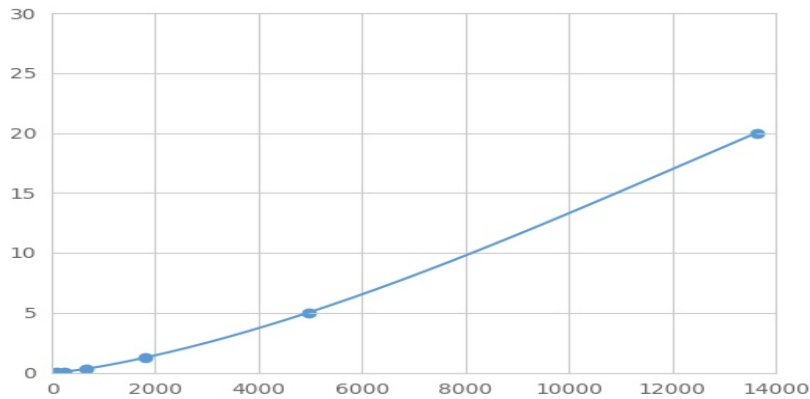
Typical Standard Curve for ABCC6 Magnetic Luminex Assay.
