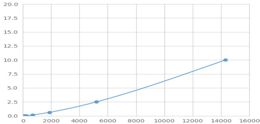
Typical Standard Curve for ATP5b Magnetic Luminex Assay.
