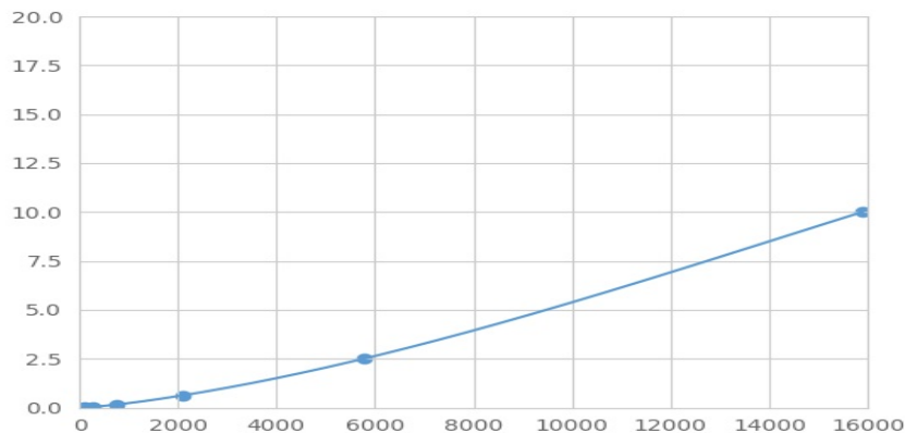
Typical Standard Curve for ARPC4 Magnetic Luminex Assay.
