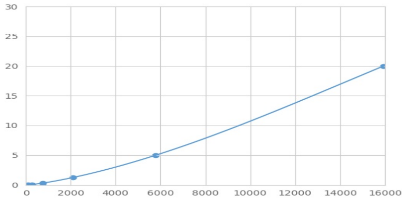
Typical Standard Curve for ATF6 Magnetic Luminex Assay.
