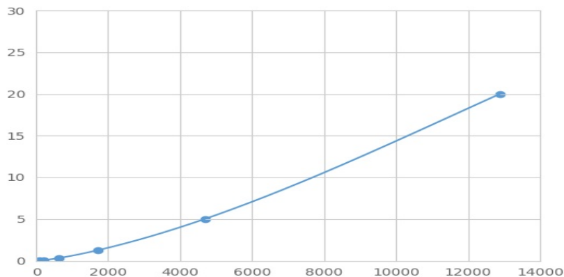
Typical Standard Curve for ADCY10 Magnetic Luminex Assay.
