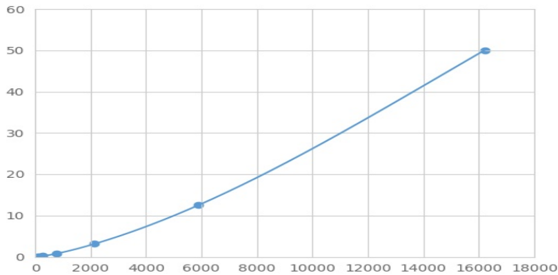
Typical Standard Curve for ADH4 Magnetic Luminex Assay.
