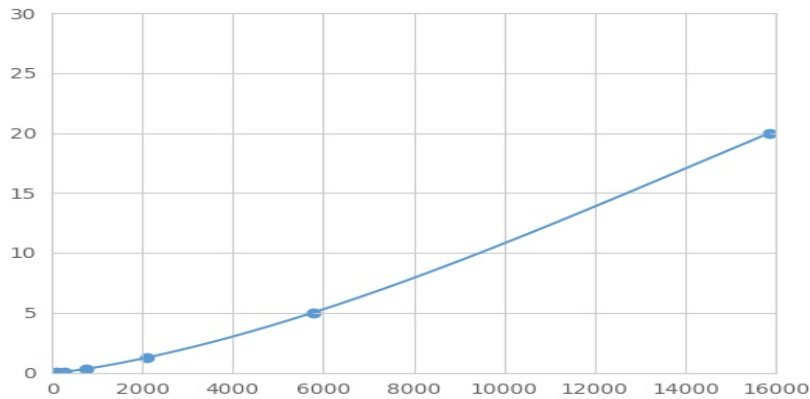
Typical Standard Curve for ALPL Magnetic Luminex Assay.
