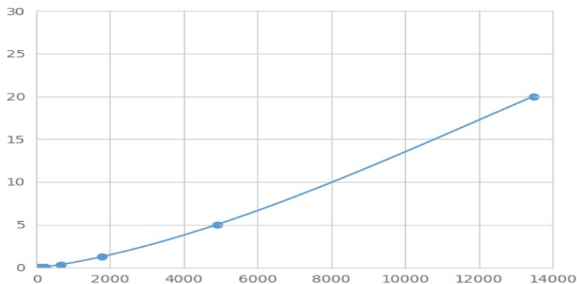
Typical Standard Curve for a1BG Magnetic Luminex Assay.
