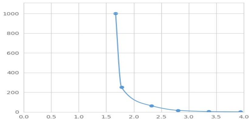
Typical Standard Curve for Ab1-40 Magnetic Luminex Assay.
