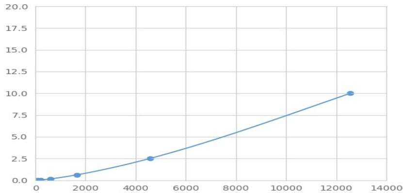
Typical Standard Curve for APLP2 Magnetic Luminex Assay.
