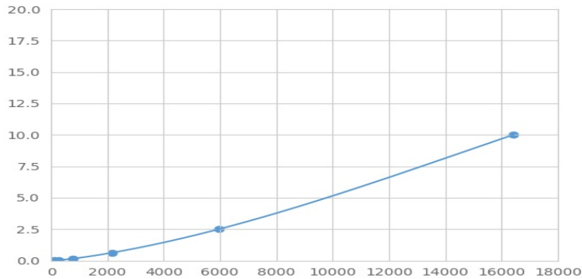
Typical Standard Curve for ANXA2 Magnetic Luminex Assay.
