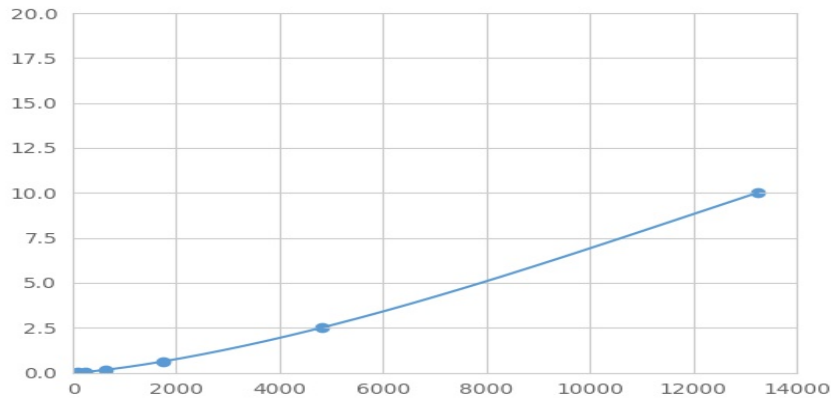
Typical Standard Curve for ANXA3 Magnetic Luminex Assay.
