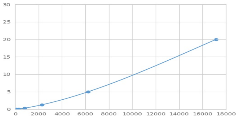
Typical Standard Curve for ANXA5 Magnetic Luminex Assay.
