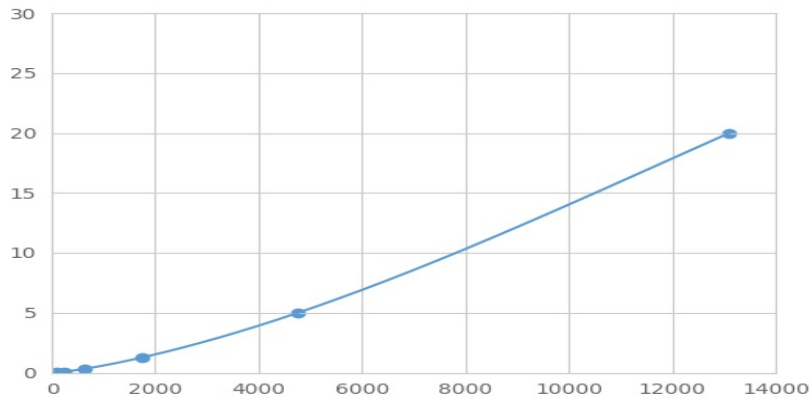
Typical Standard Curve for ANTXR2 Magnetic Luminex Assay.
