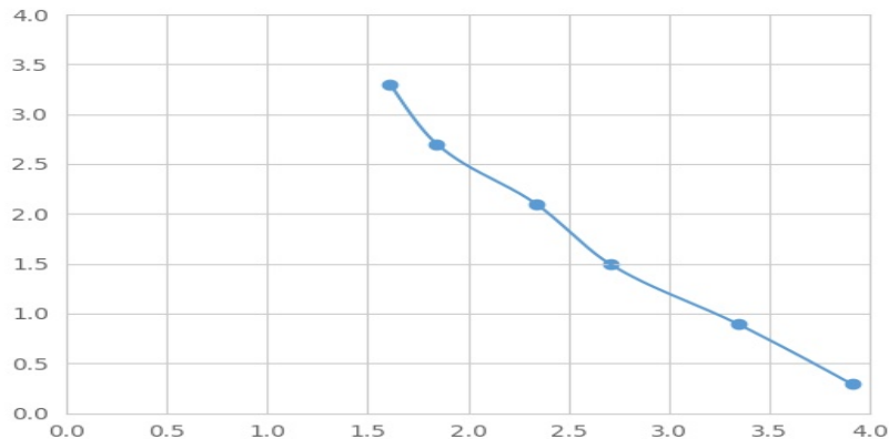
Typical Standard Curve for APOA1 Magnetic Luminex Assay.
