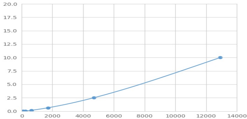
Typical Standard Curve for APOB Magnetic Luminex Assay.
