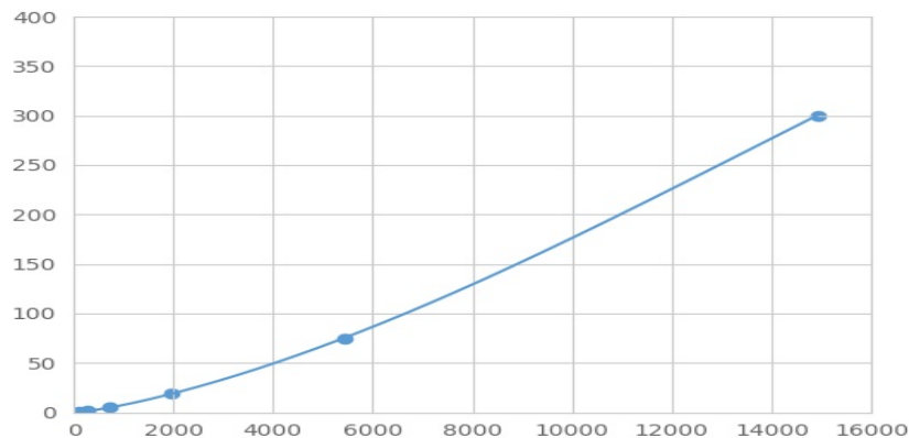
Typical Standard Curve for APOC1 Magnetic Luminex Assay.
