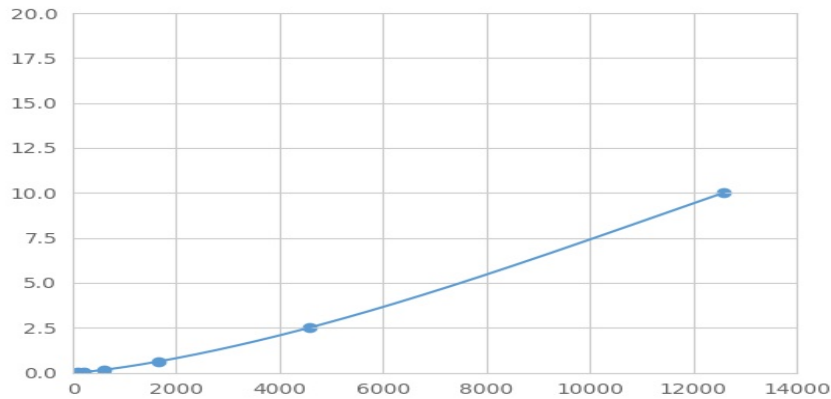
Typical Standard Curve for BST2 Magnetic Luminex Assay.
