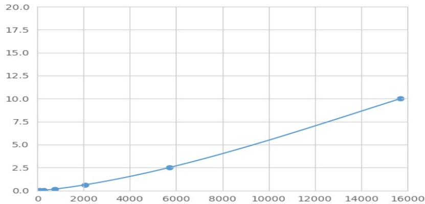
Typical Standard Curve for BDKRB2 Magnetic Luminex Assay.
