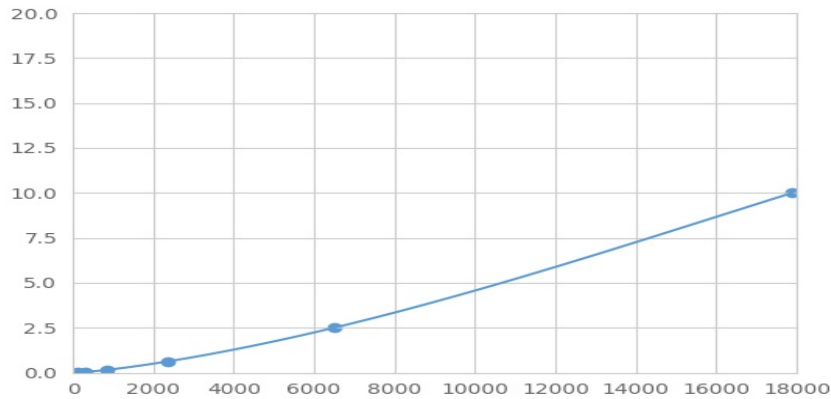
Typical Standard Curve for BCAS4 Magnetic Luminex Assay.
