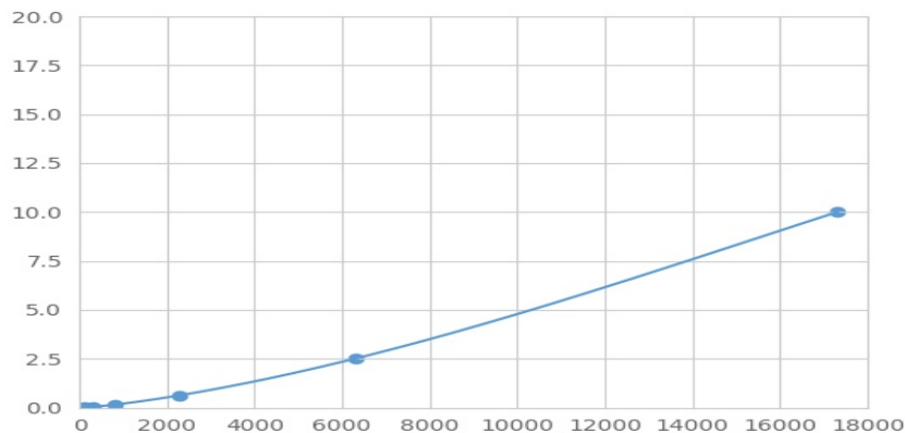
Typical Standard Curve for BTN1A1 Magnetic Luminex Assay.
