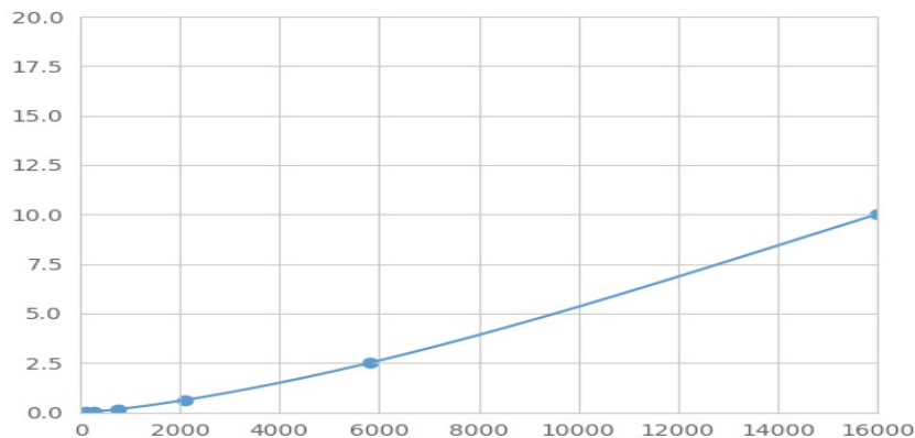
Typical Standard Curve for CALML3 Magnetic Luminex Assay.
